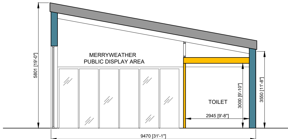
TYPICAL SECTION B-B SCALE 1:100
