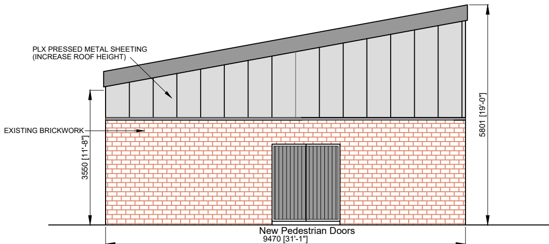
PROPOSED SIDE ELEVATION (East) SCALE 1:100
