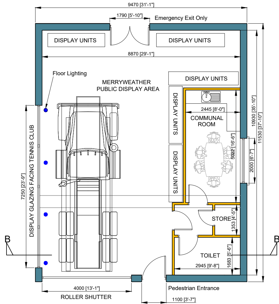
PROPOSED FLOOR PLAN SCALE 1:100 - 96sqm
