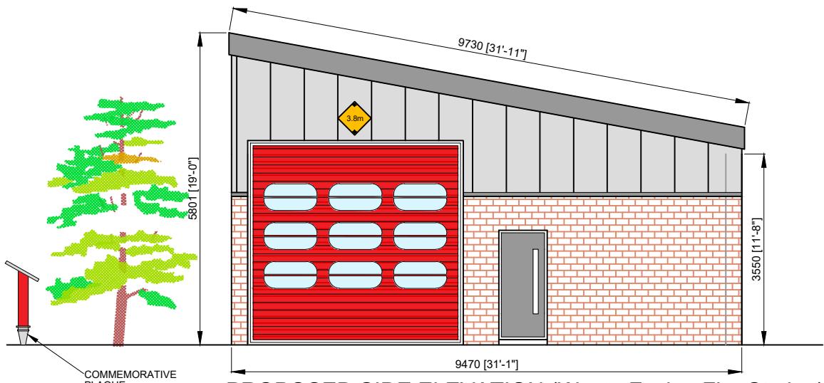
PROPOSED SIDE ELEVATION (West - Facing Fire Station) SCALE 1:100
