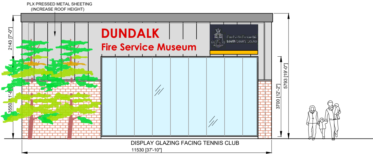
PROPOSED FRONT ELEVATION (North - Facing Tennis Courts / Ramparts) SCALE 1:100
