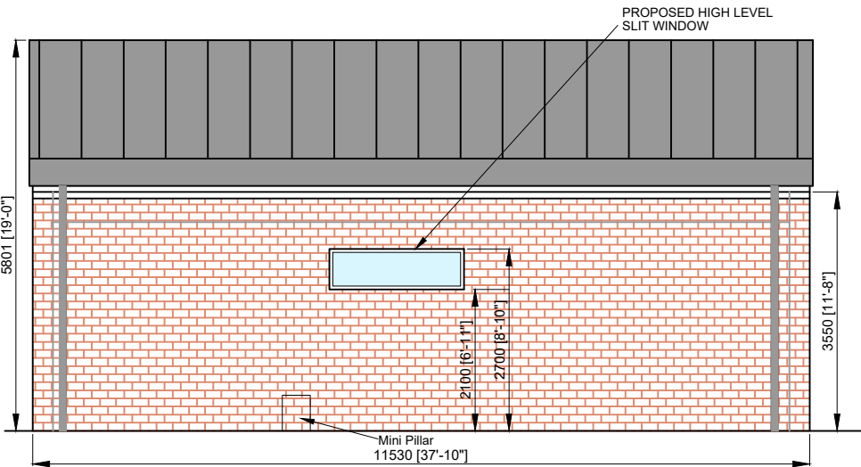
PROPOSED REAR ELEVATION (South - facing green area) SCALE 1:100
