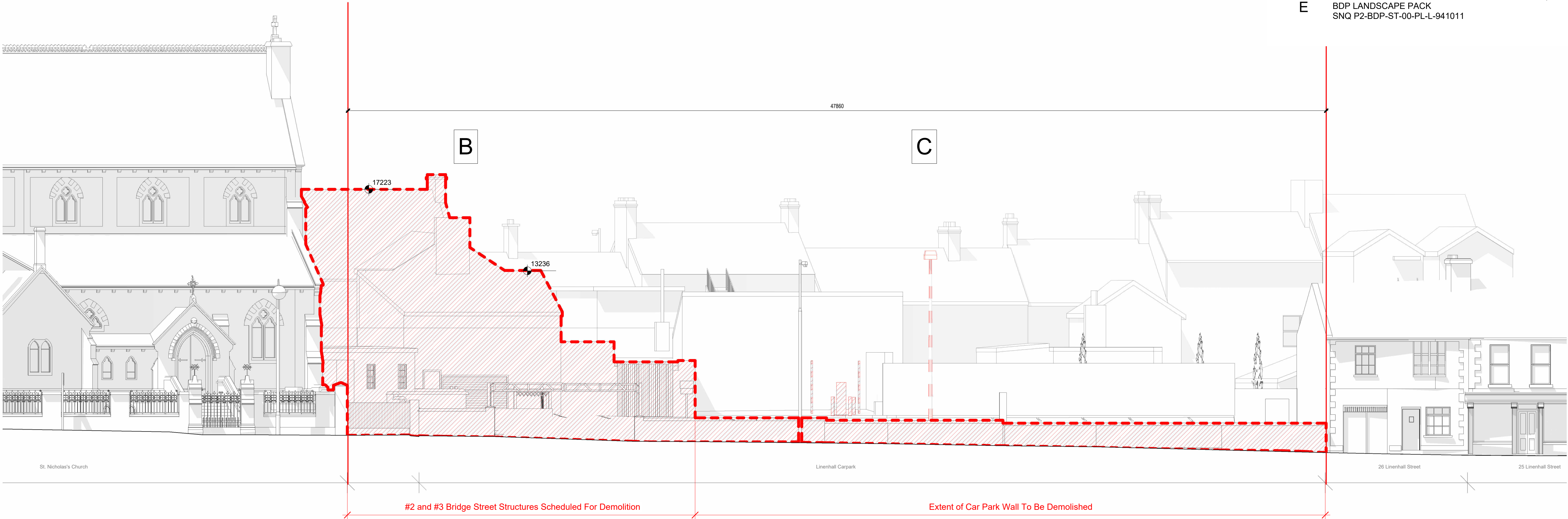
Demolition Elevation Existing Linenhall Street 1:100
