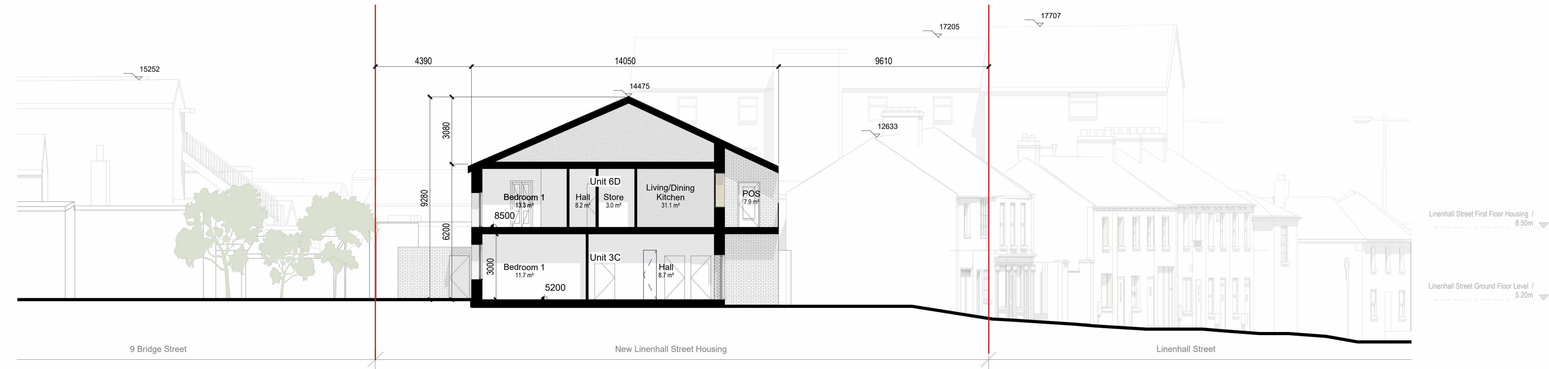
Residential Unit Proposed Section CC 1:100
