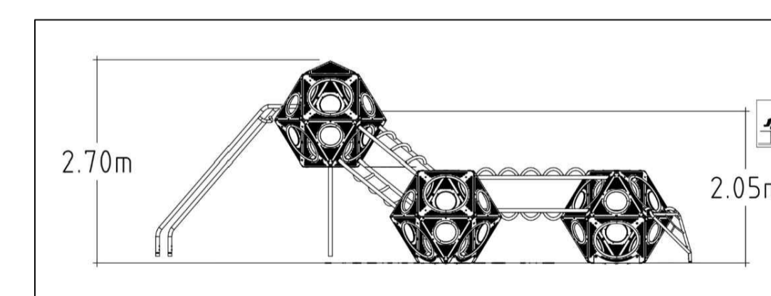
Proposed 1no Hags - Playcube Ara
