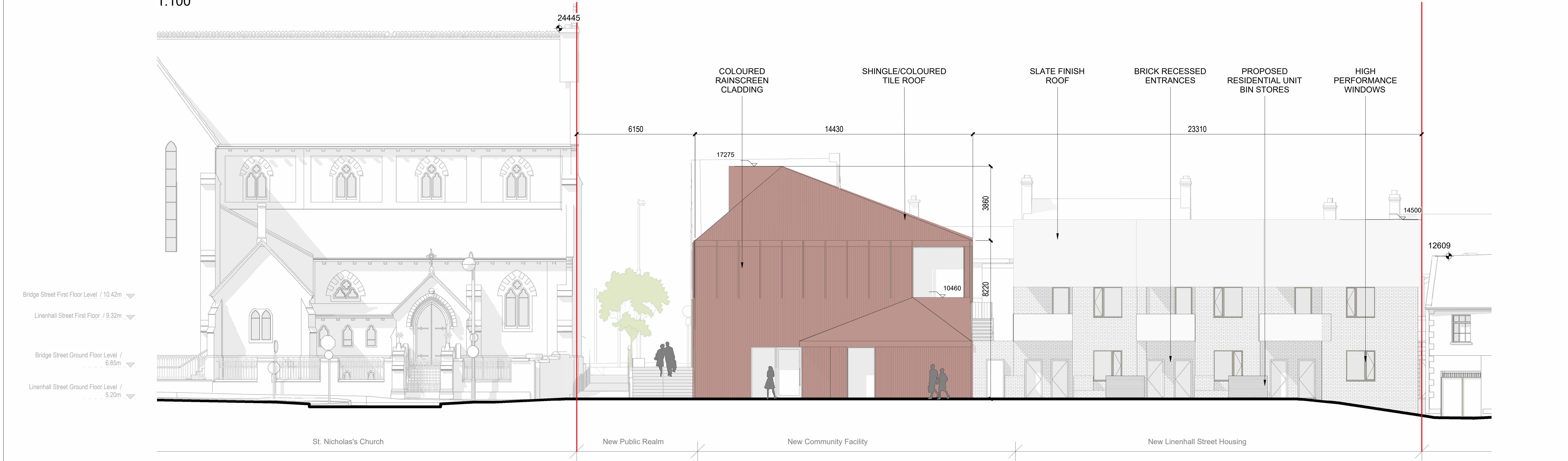
Community Facility Proposed Linenhall Street Elevation 1:100
