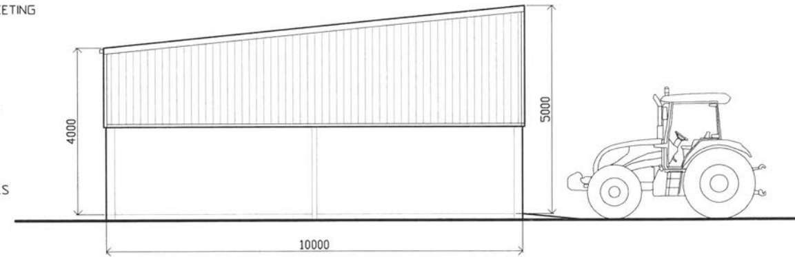
Eastern Elevation
