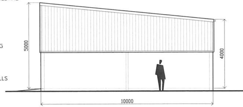
Western Elevation
