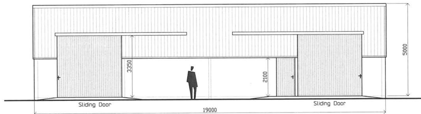
Northern Elevation
