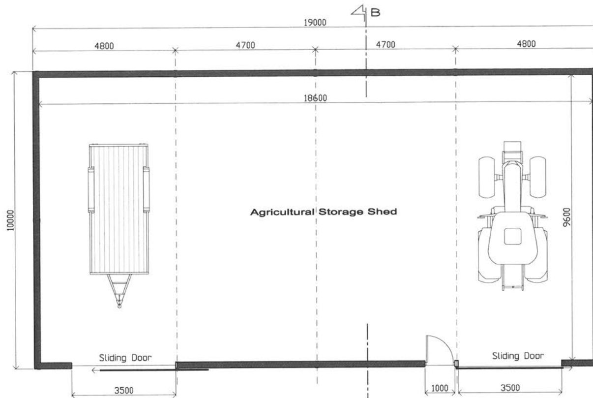
Floor Plan
