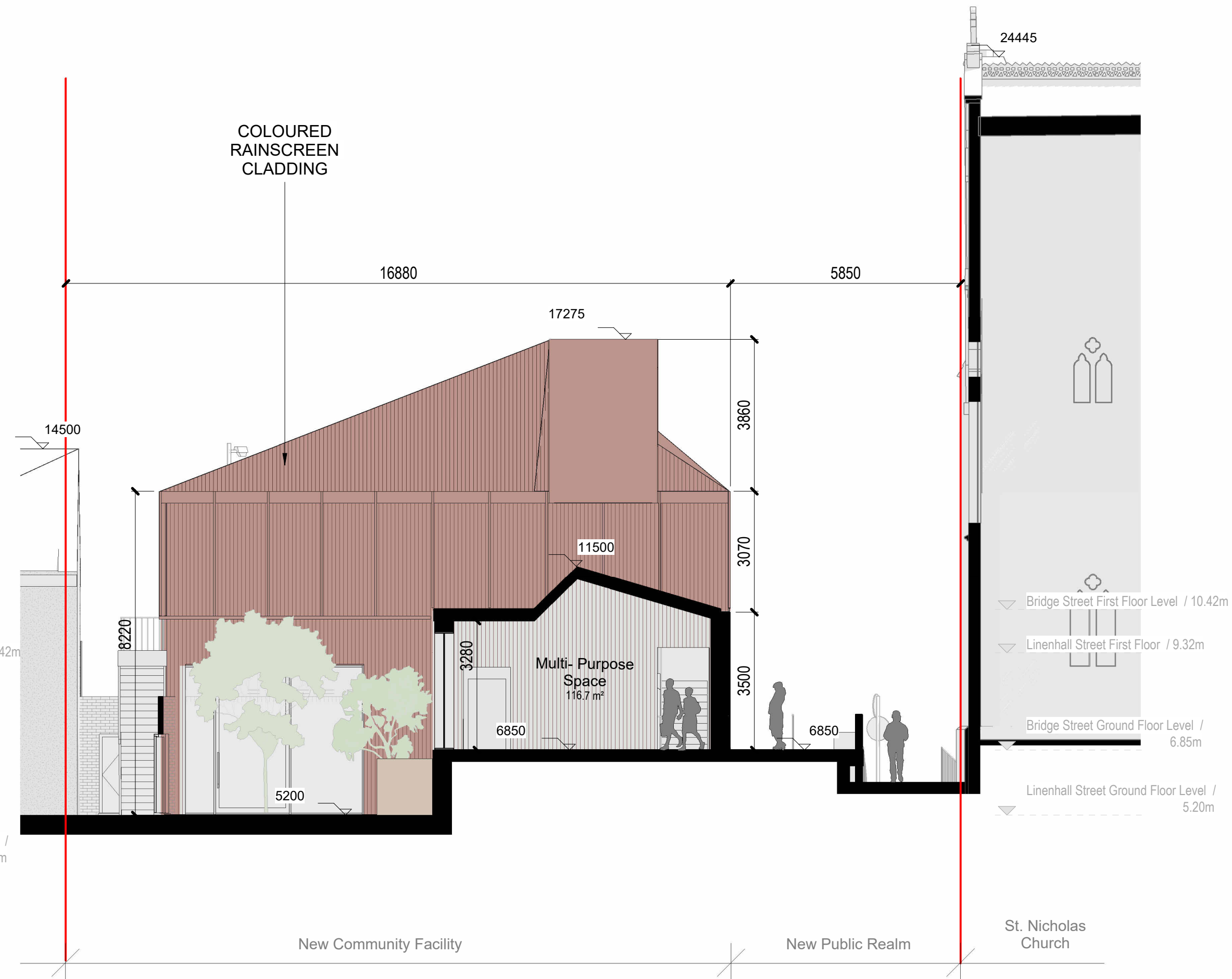
Community Facility Proposed Section BB 1:100
