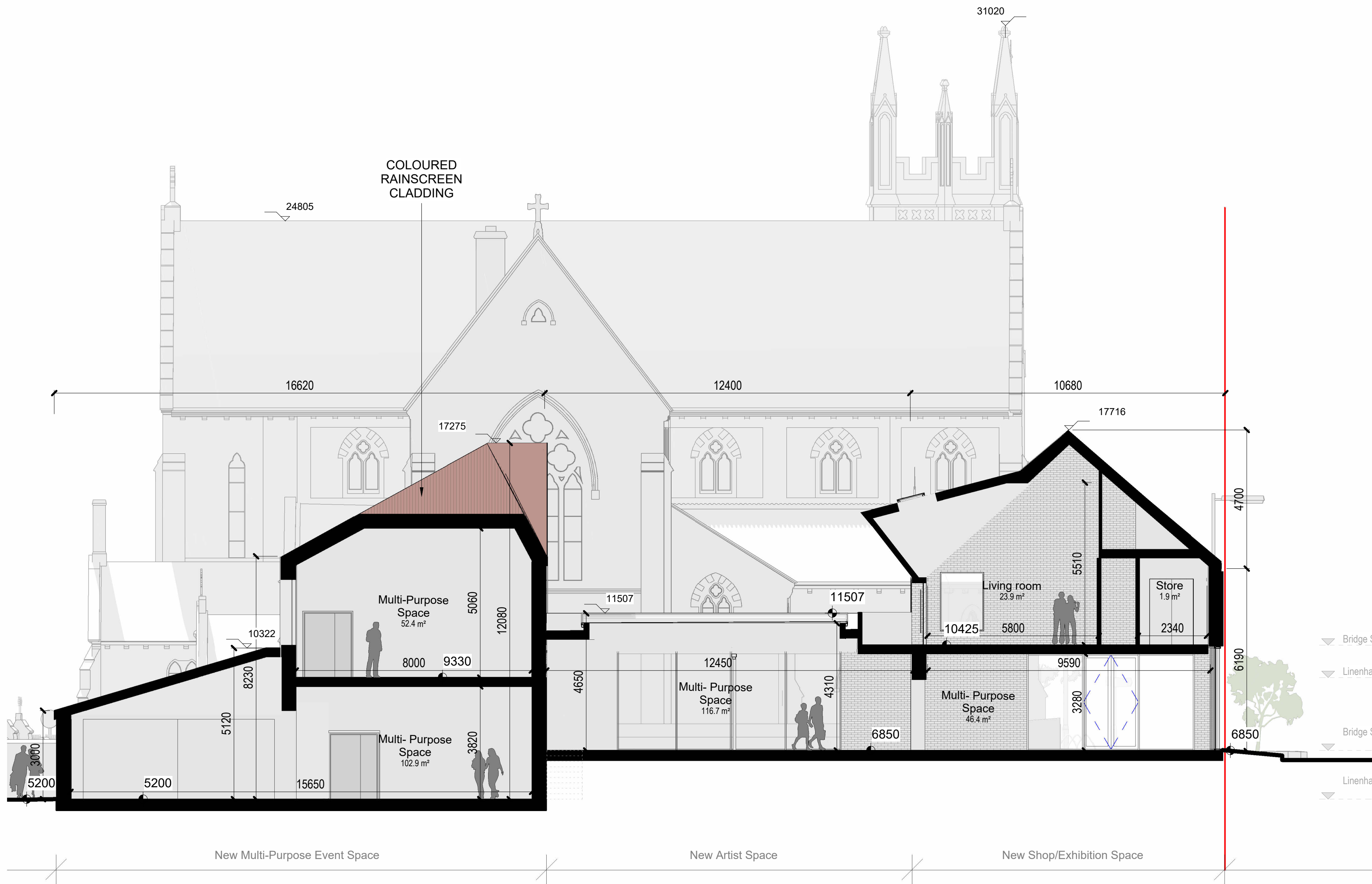
Community Facility Proposed Section AA 1:100
