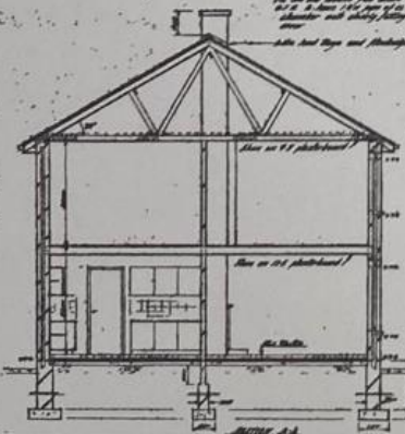
CROSS SECTION
